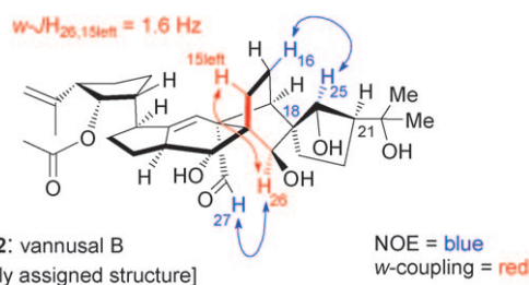
Figure 2. Key 1 H NMR coupling constant ( w\text{-}J_{H_{26}, 15\text{left}} = 1.6 \text{ Hz} ) and NOE interaction exhibited by both the originally assigned structure (synthetic, 2 ) and natural vannusal B.
