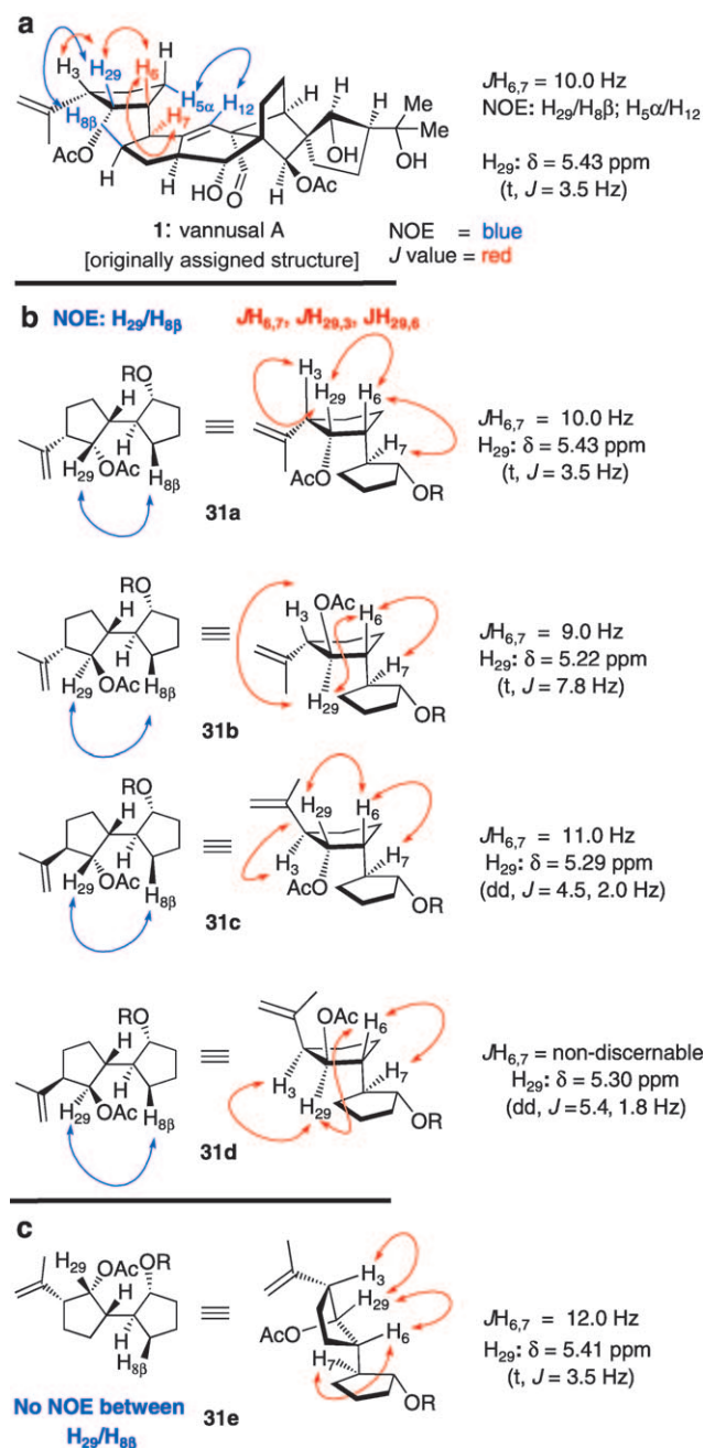
Figure 6. Relevant NOE interactions and coupling constants ( J ) of AB-ring model compounds 31a–31e. R = TBDS = tert -butyldiphenylsilyl.
